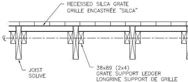
Figure 2: Section A
